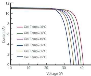
Current-Voltage Curve
