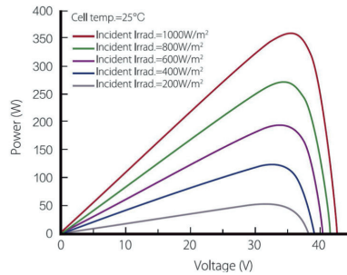
Power-Voltage Curve
